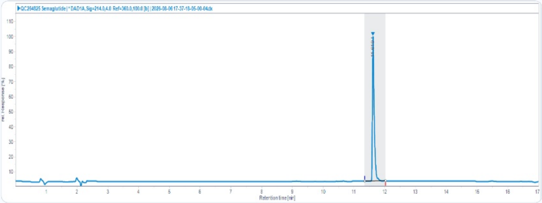
HPLC Chromatogram (Retention Time: 11.619 min)
